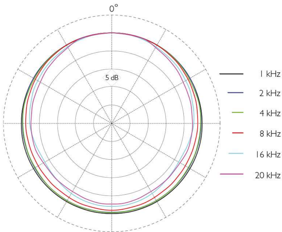
Typical response of a 4071
