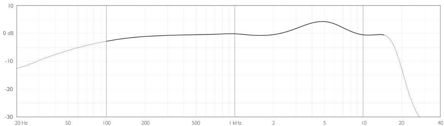
Typical response of a 4071
