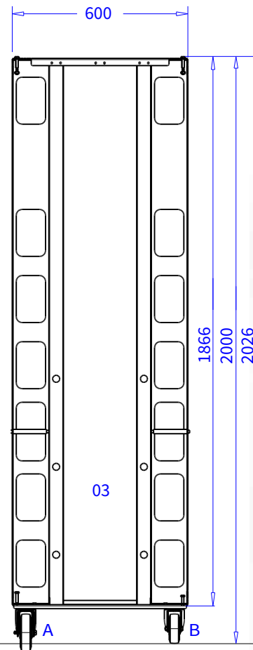
Fork-side panel H203xW60 WAM2P61 - single panel WAFSF21A set of 2 (incl. boltset) WAFSF21B centre bracket, set of 2 (incl. boltset)
