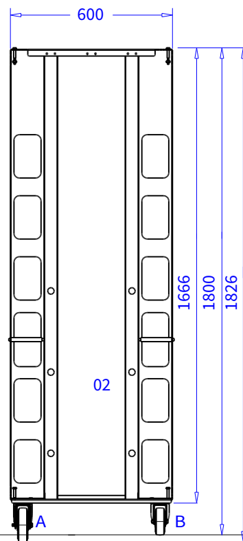
Fork-side panel H183xW60 WAM2P80 - single panel WAFSF15A set of 2 (incl. boltset) WAFSF15B centre bracket, set of 2 (incl. boltset)
