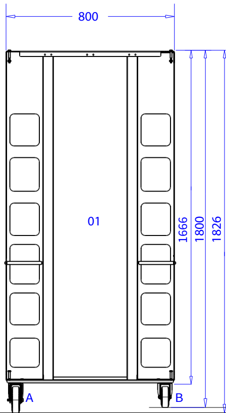
Fork-side panel H183xW80 WAM2P86 - single panel WAFSF17A - set of 2 (incl. boltset) WAFSF17B - centre bracket, set of 2 (incl. boltset)
