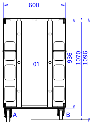
Fork-side panel H110xW60 WAM2P60 - single panel WAFSF11A set of 2 (incl. boltset) WAFSF11B centre bracket, set of 2 (incl. boltset)
