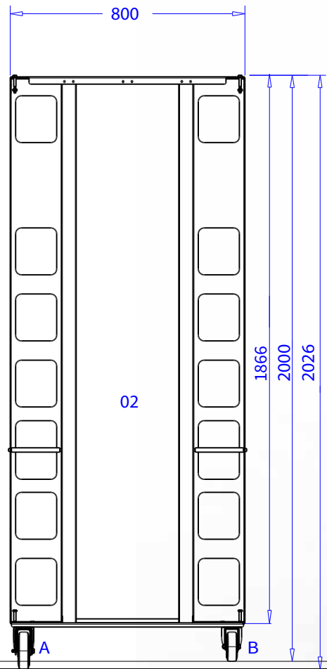
Fork-side panel H203xW80 WAM2P62 - single panel WAFSF31A - set of 2 (incl. boltset) WAFSF31B - centre bracket, set of 2 (incl. boltset)
