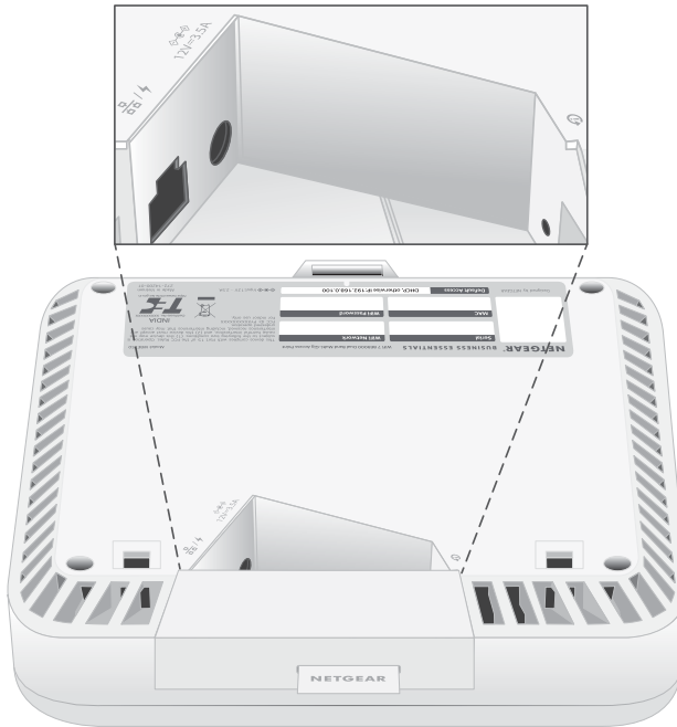
Figure 2. Hardware interfaces
