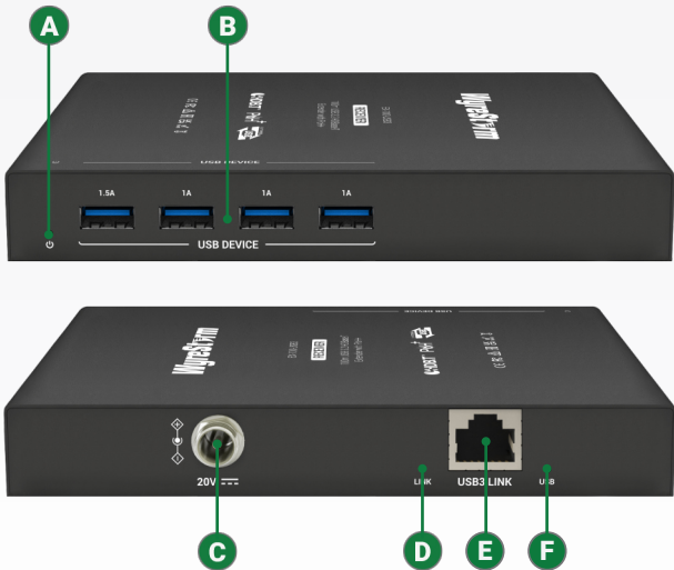
EX-100-USB3 (Rear)
