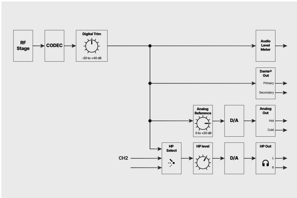
Trimming of the digital Receiver (one channel).
